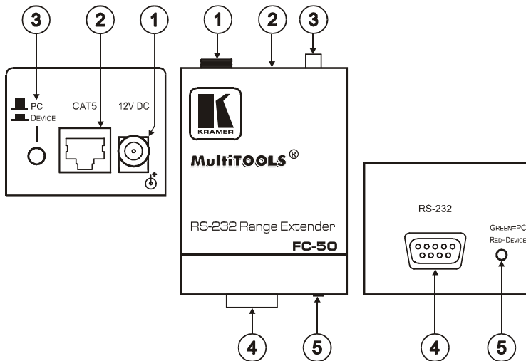
Figure 1: FC-50 RS-232 Range Extender
