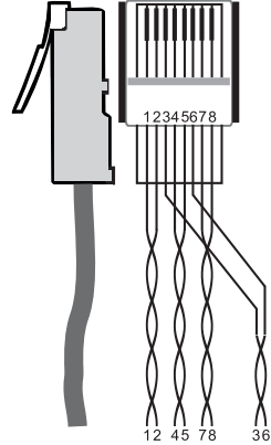
Figure 4: CAT 5 PINOUT
