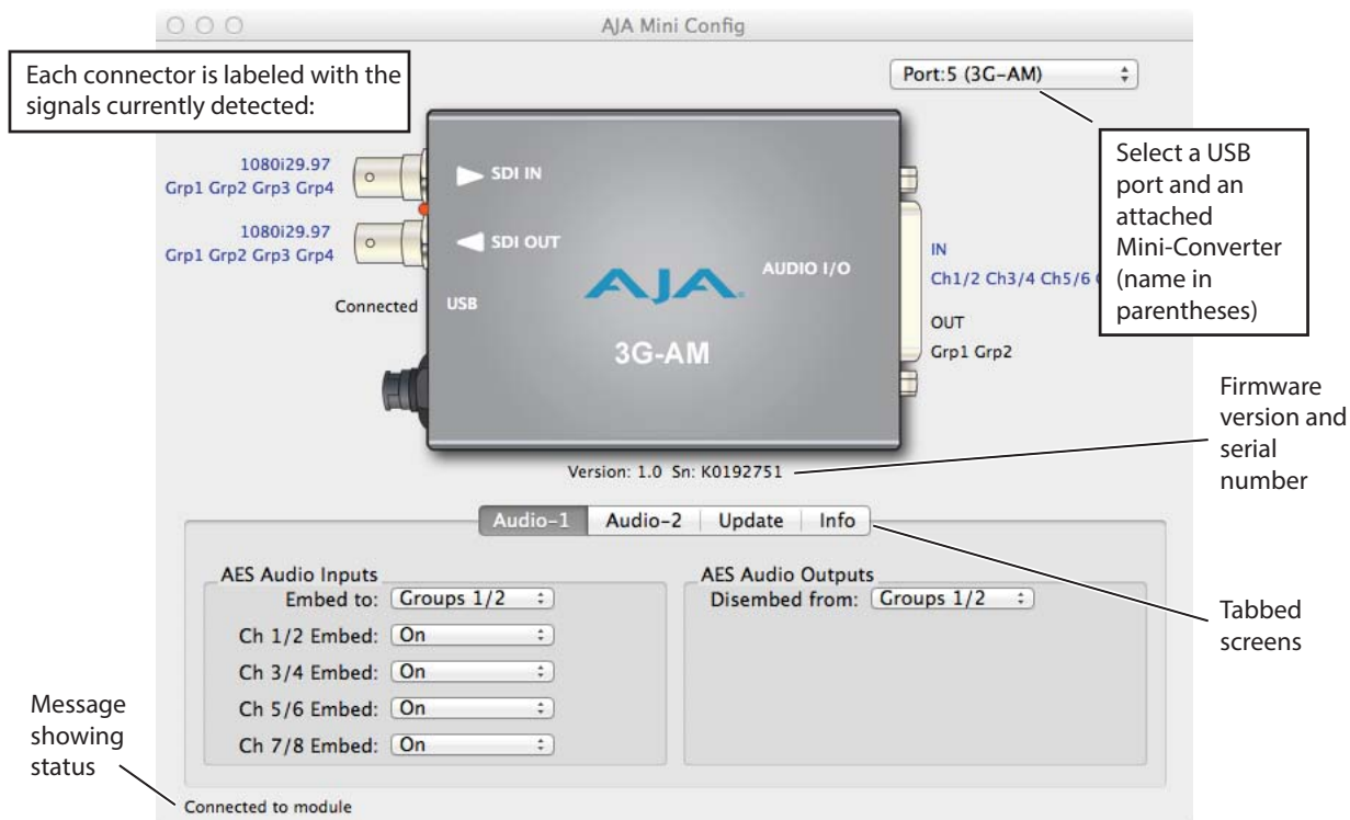
Figure 6. MiniConfig Screen
