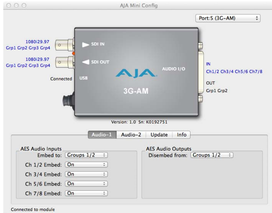
Figure 7. MiniConfig, Audio-1 Tab Screen
