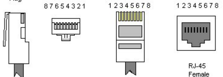
RJ-45 Male Plug
