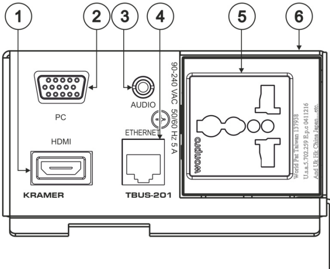
Figure 3: TBUS-201xl Connecting Surface
