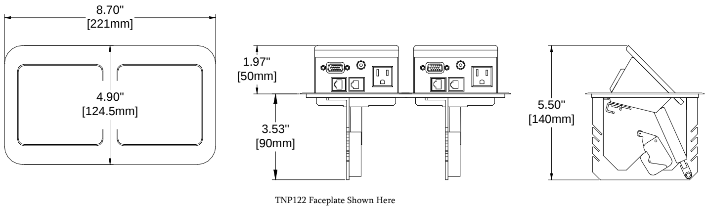
Diagram 3: Dual Unit Dimensions (TNP122, TNP142)
