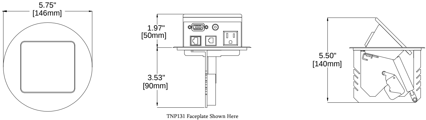
Diagram 1: Round Bezel Dimensions (TNP126, TNP126C, TNP131, TNP141, TNP141C)
