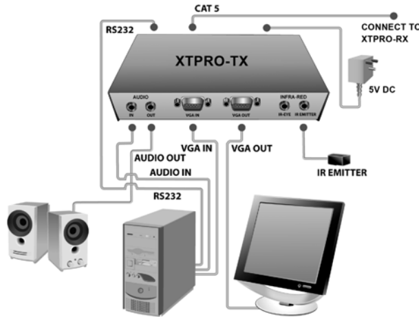
XTPRO Transmitter Installation Diagram
