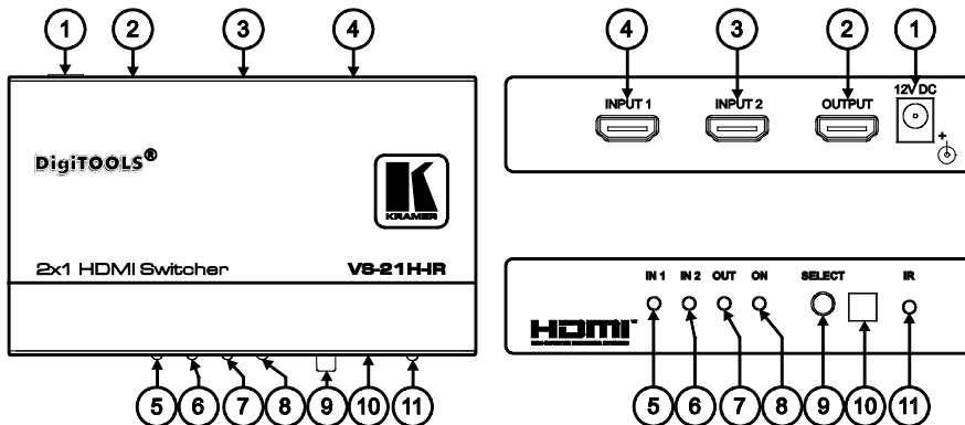
Figure 1: VS-21H-IR 2x1 HDMI Switcher
