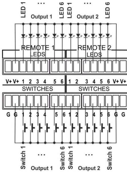
Figure 7: Remote Contact-closure Switch and LED Connections
