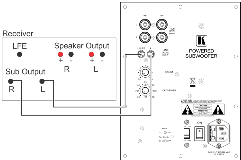
Figure 5: Connecting via Line Input
