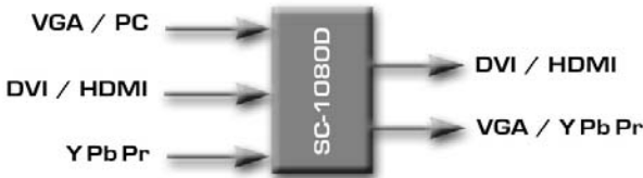
Figure 1 – Block Diagram
