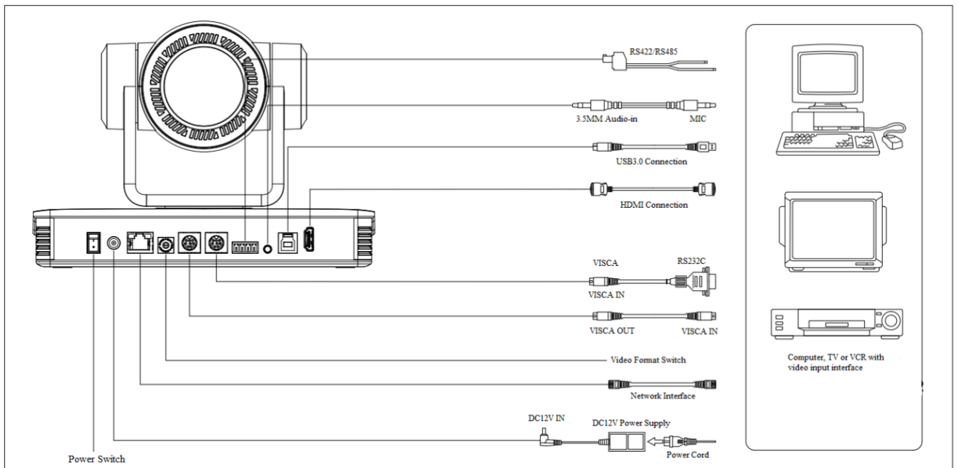
Figure 2.5 Wiring Diagram
