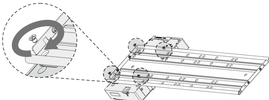
Figure 2-7 Fix the HDD (1)
