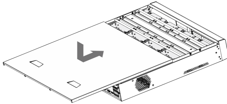
Figure 2-11 Complete installation
