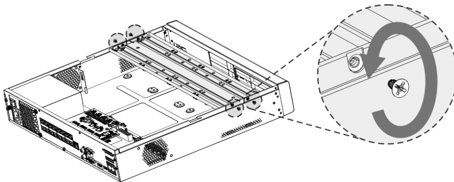
Figure 2-6 Remove HDD bracket (4-HDD)
