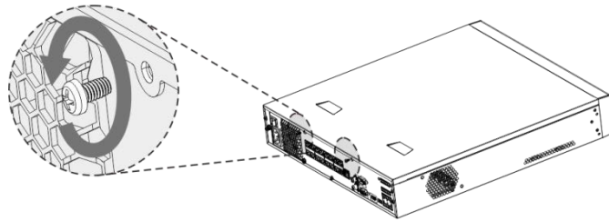
Figure 2-5 Remove case cover
