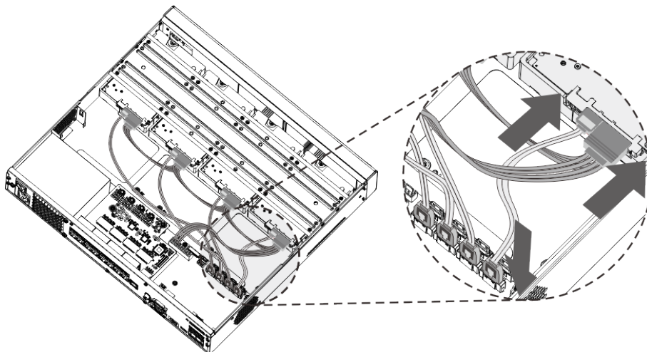
Figure 2-10 Connect cables
