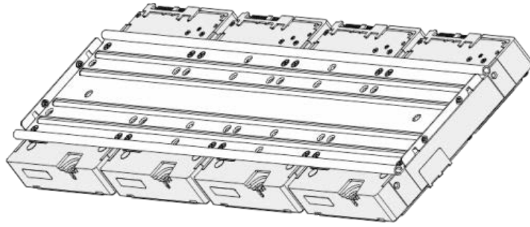
Figure 2-9 Fasten HDD bracket
