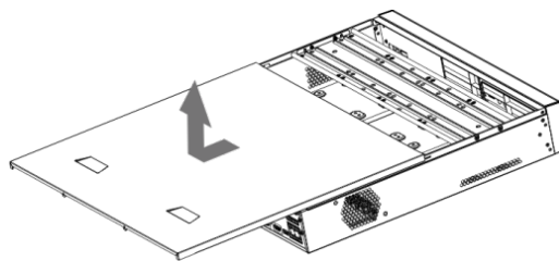
Figure 2-5 Remove case cover
