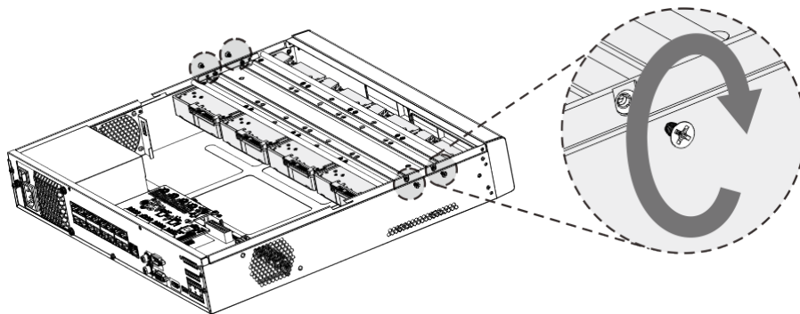
Figure 2-9 Fasten HDD bracket
