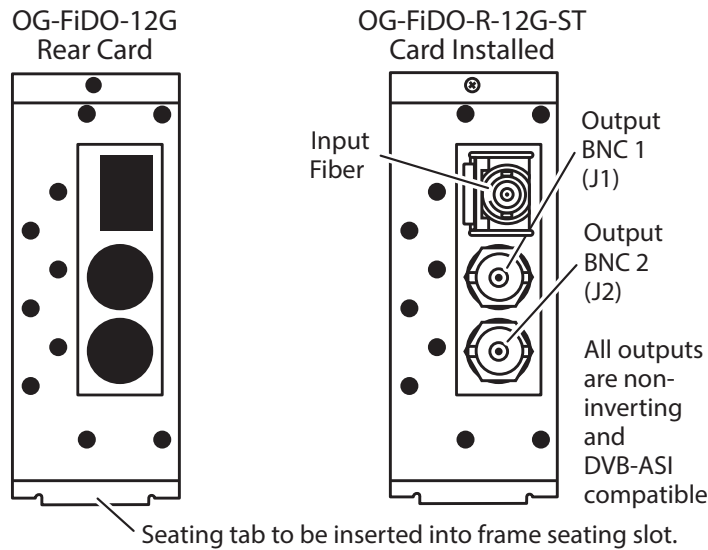
Figure 2. Rear View of Empty Rear Card and Installed Single Channel FiDO Cards
