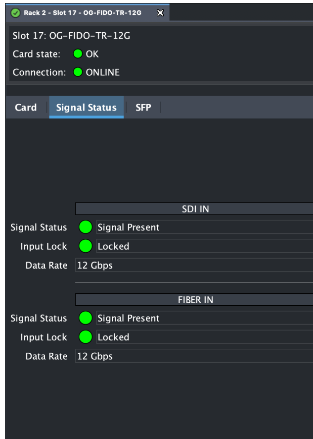
Figure 14. OG-FiDO-12G Series Signal Status Tab Screen in Dashboard
