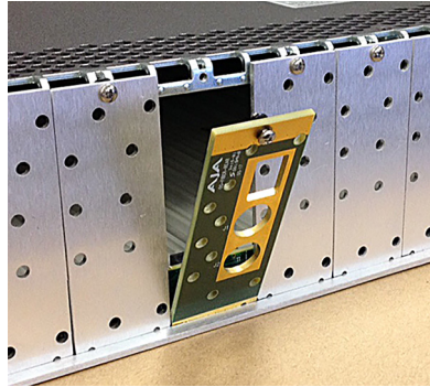
Figure 5. Rear Card Inserted Into Frame Seating Slot
