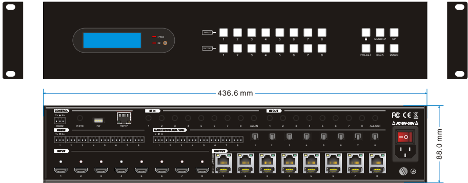
Matrix Switch
