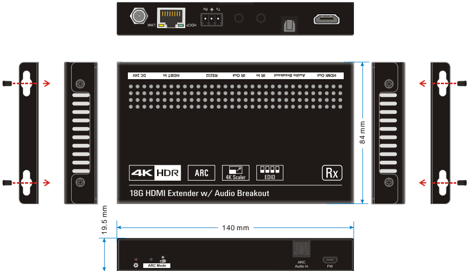
HDBaset Receiver
