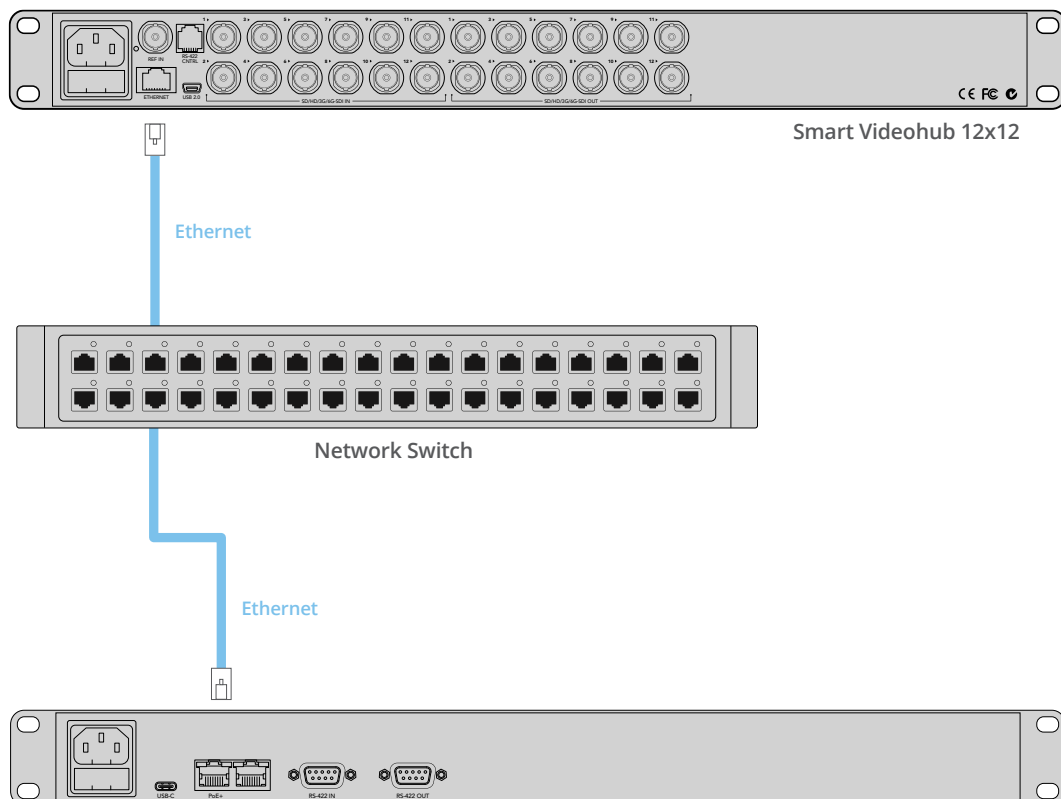
Videohub Smart Control Pro connected to a Smart Videohub 20x20 via an Ethernet Network Switch.
