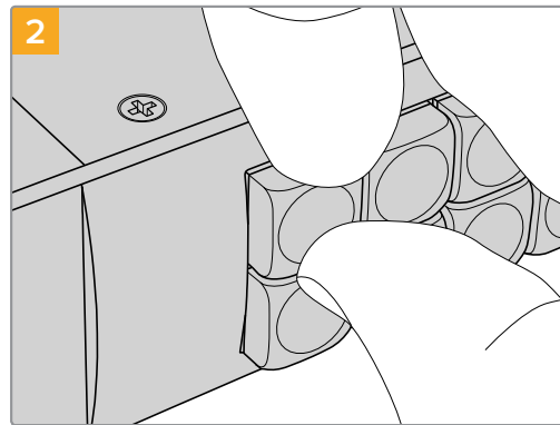
2 The button keycaps can be easily removed by inserting your fingernail between the keycap and the button.
