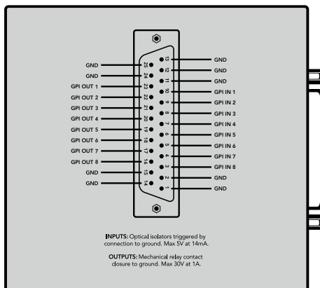
Pinout diagram of the DB25 connector
