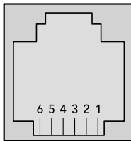
Videohub RS-422 Router Control RJ11 pinout diagram.
