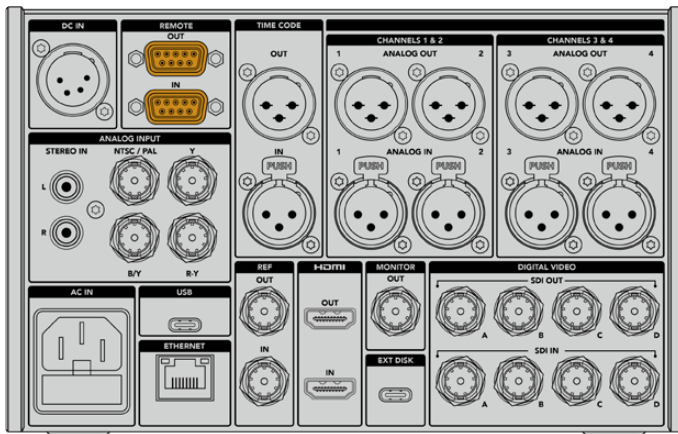
REMOTE-Anschlüsse am HyperDeck Extreme 8K HDR
