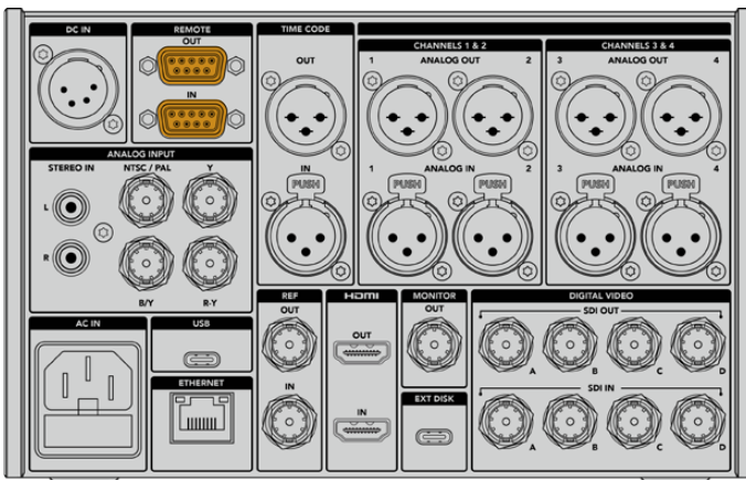
Porta remota do HyperDeck Extreme 8K HDR.
