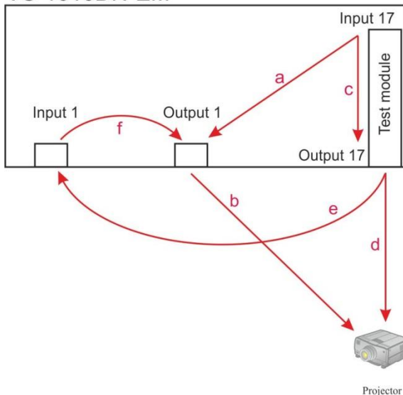
Figure 16: Signal Paths for Isolating Video Problems
