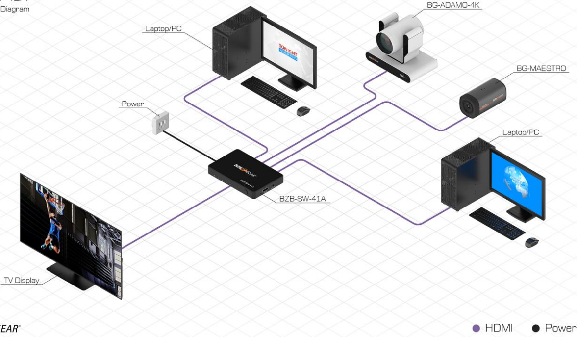
BZB-SW-41A Connection Diagram
