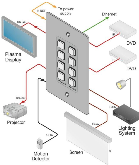
Figure 2: Connecting the RC-76R/RC-78R Room Controllers
