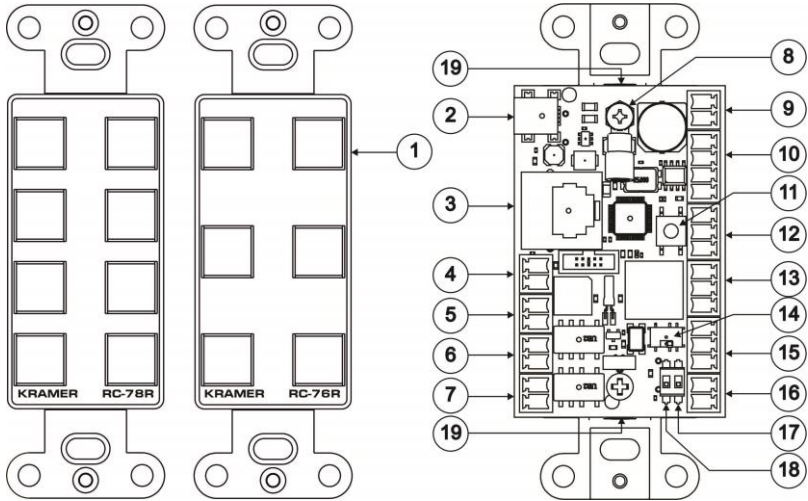
Figure 1: RC-76R/RC-78R Room Controllers
