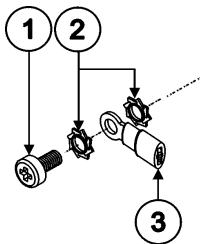
Figure 4: Grounding Connection Components
