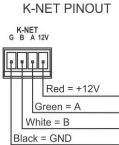
Figure 3: K-NET PINOUT Connection
