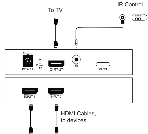
Connection Diagram
