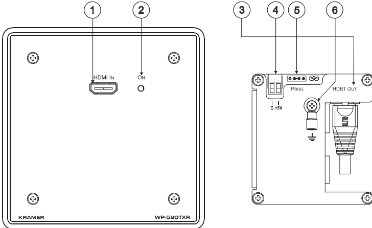
Figure 1: WP-580Txr HDMI Line Transmitter for the US
