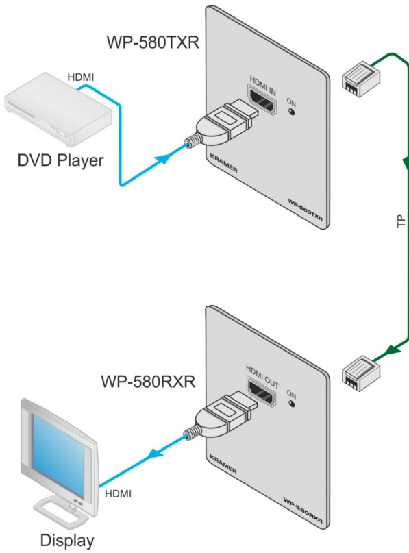
Figure 5: Connecting the WP-580Txr/WP-580Rxr Transmitter/Receiver Pair
