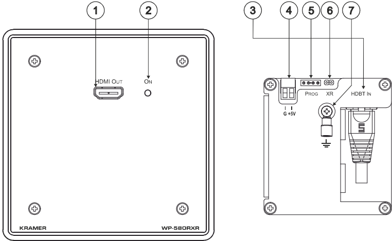
Figure 3: WP-580Rxr HDMI Line Receiver for the US
