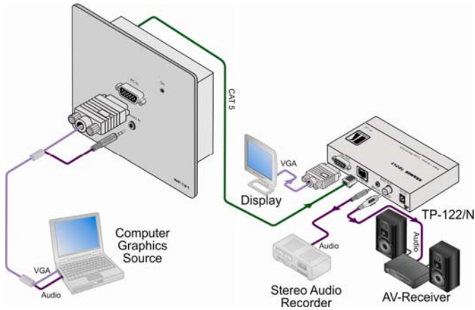
Figure 4: Installing and Connecting the WP-121
