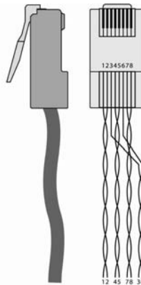
Figure 6: CAT 5 PINOUT
