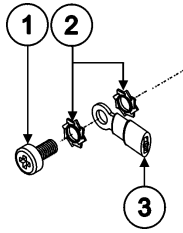
Figure 5: Ground Connection
